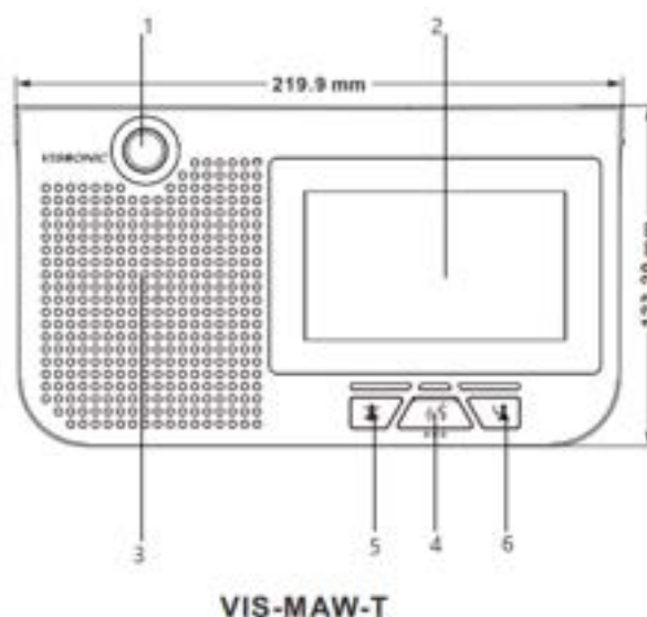
Figure 3.7.1.1 Top view of VIS-MAW-T
