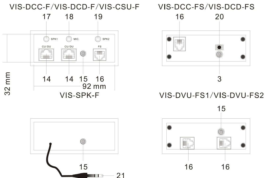
Figure 3.5.1.2 Rear view of VIS-DCC/DCD/CSU/DVU/SPK-F/FS/FS1/FS2
