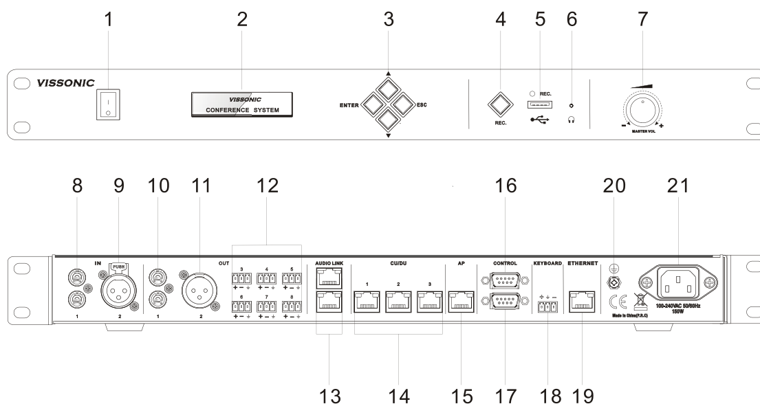
Figure 2.1.1 VIS-DCP2000-D/W front and rear panels
