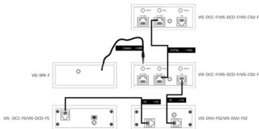
Figure 3.5.3 Connection of VIS-DCC/DCD/CSU/DVU/SPK-F/FS/FS1/FS2
