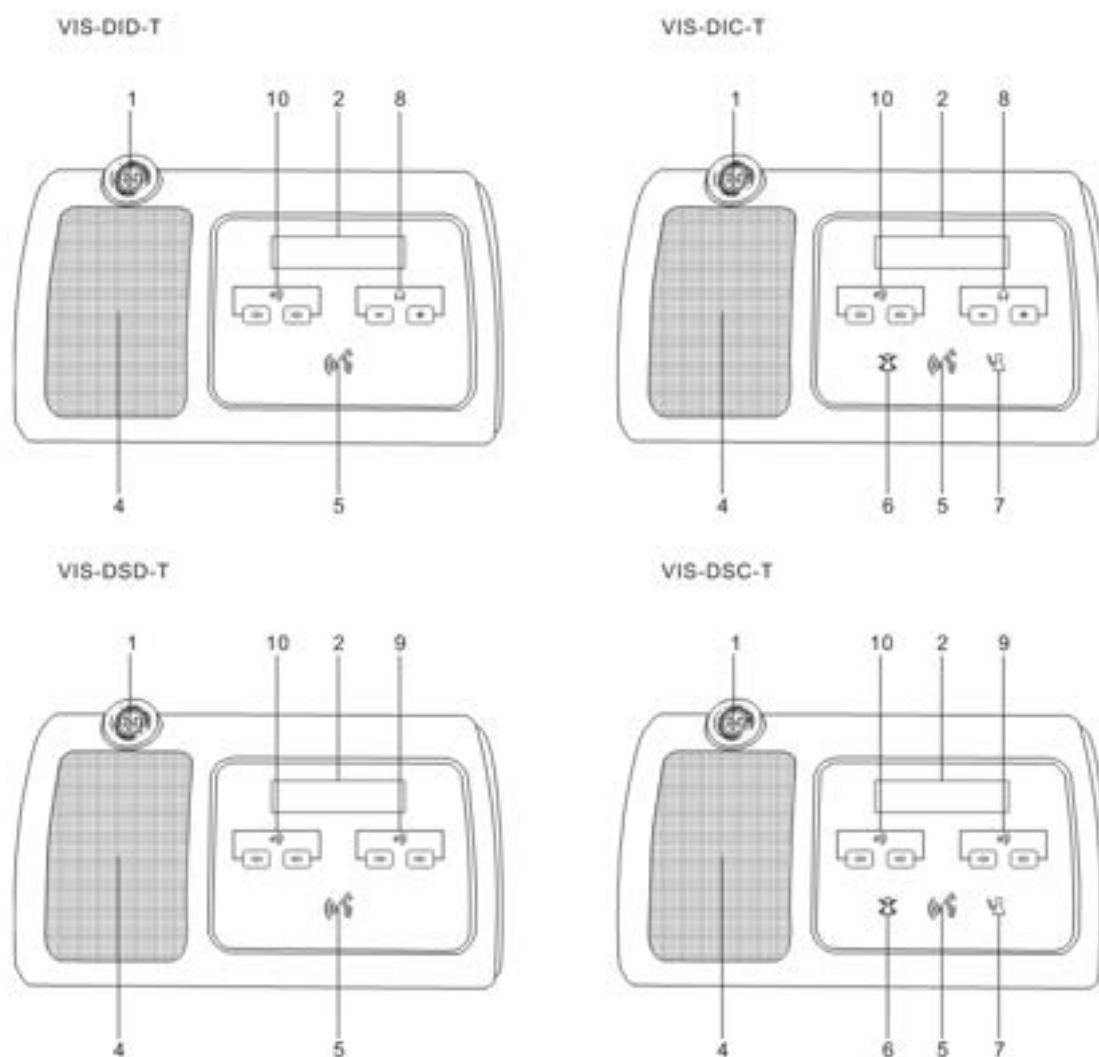
Figure 3.1.1.2 Top view of wired units VIS-DIC/DID/DSC/DSD-T
