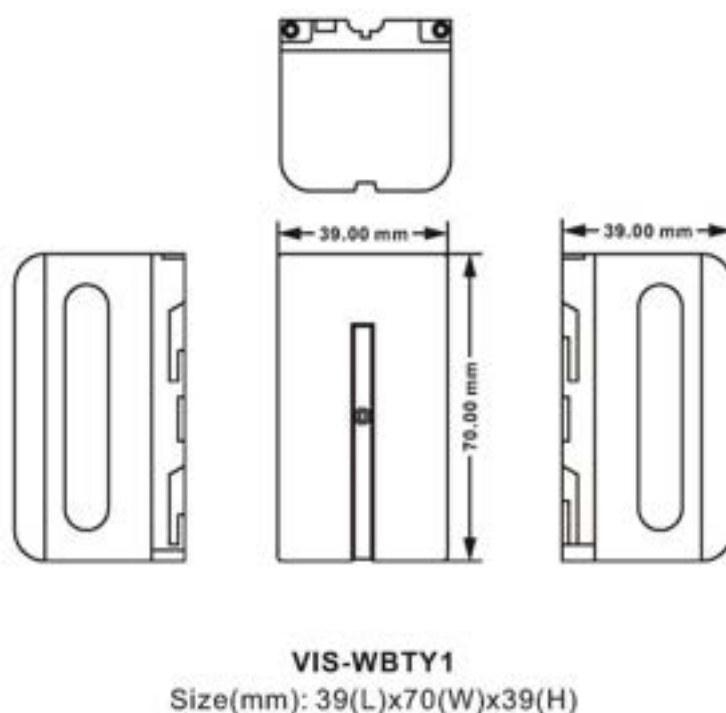
Figure 3.6.1.7 Dedicated VIS-WBTY1 battery pack
