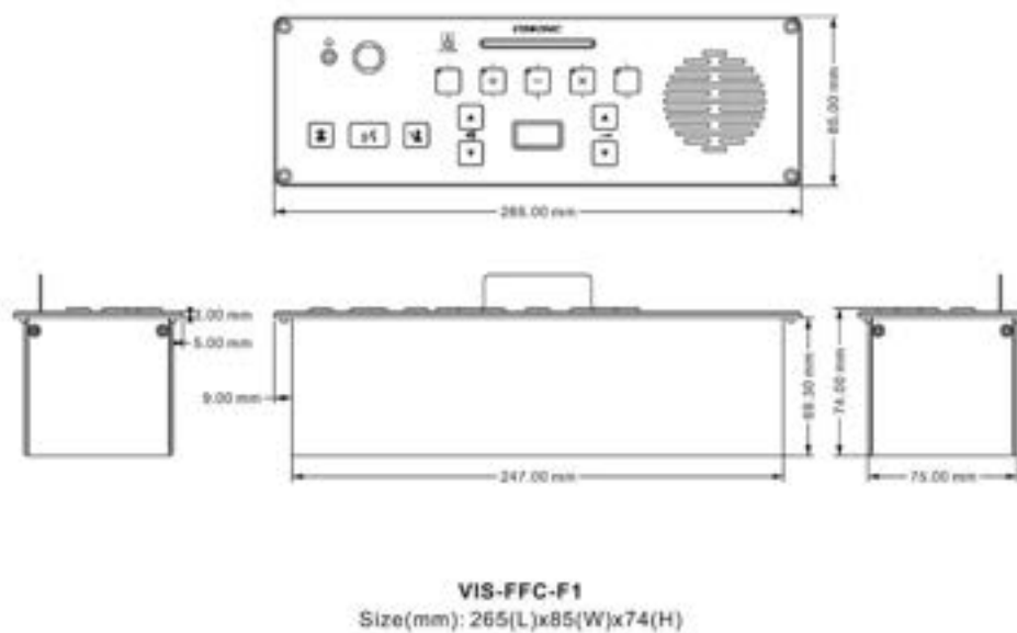
Figure 3.5.2.1.2 Sizes of VIS-FFC/FFD-F1/F2
