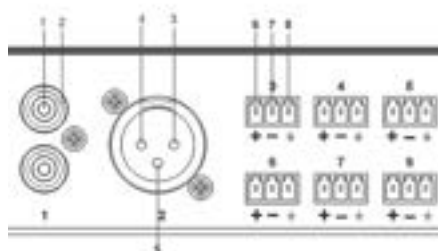
Figure 2.1.3.3 Audio output ports
