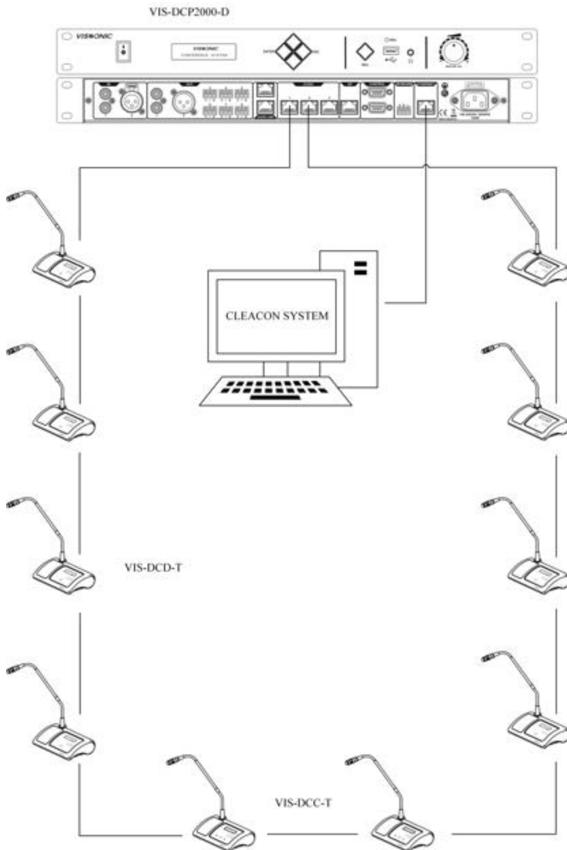
Figure 1.1.1 Wired conference system
