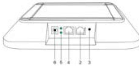
Figure 6.4.3 Ports on the side of VIS-AP4C
