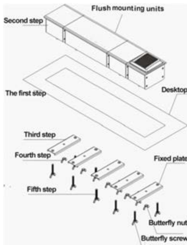
Figure 3.5.2.2 Installation steps of VIS-DCC/DCD/CSU/DVU/SPK-F/FS/FS1/FS2
