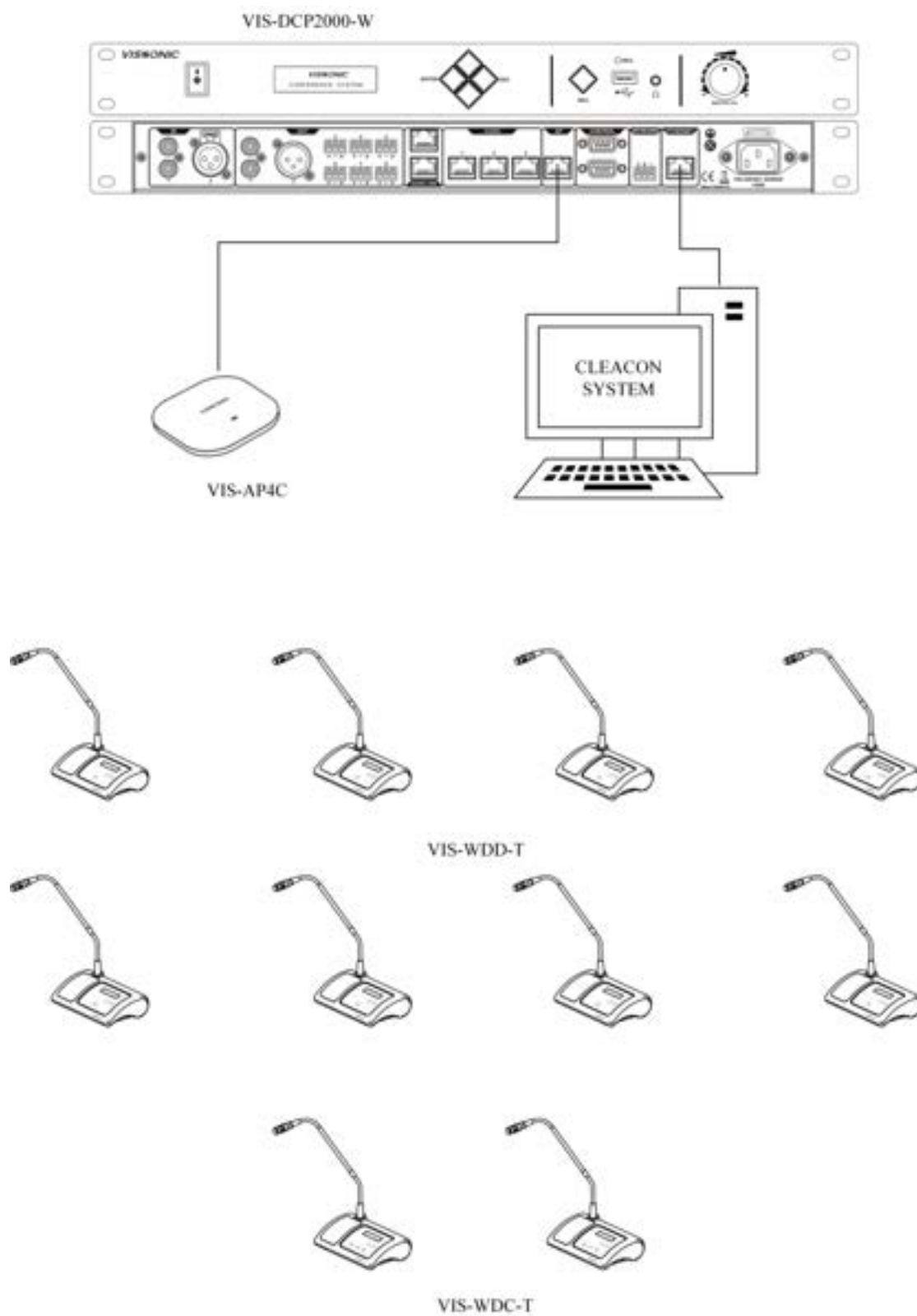
Figure 1.1.2 Wireless conference system
