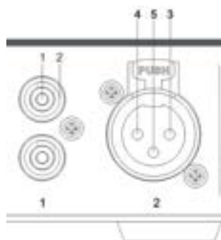
Figure 2.1.3.2 Audio input ports
