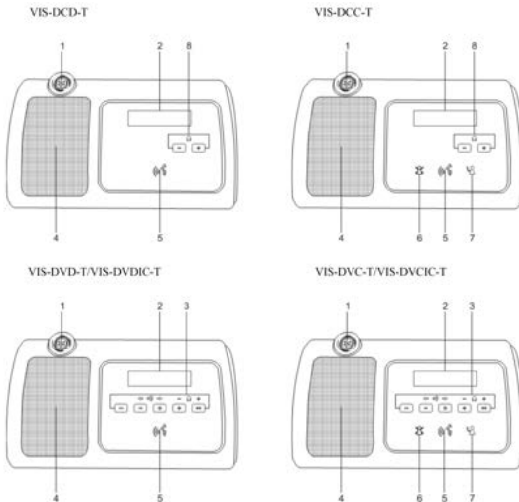
Figure 3.1.1.1 Top view of wired units VIS-DCC/DCD/DVC/DVD/DVCIC/DVDIC-T
