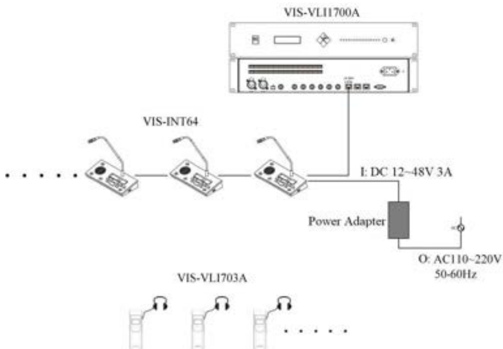
Figure 4.2.2 VIS-INT64 directly connected to infrared transmitter
