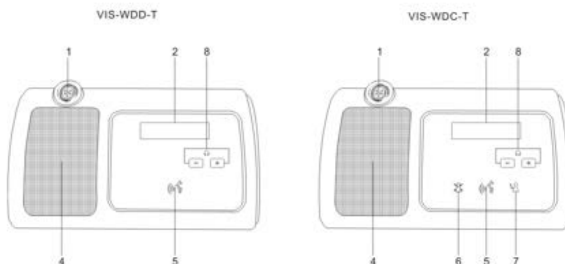
Figure 3.6.1.1 Top view of VIS-WDC/WDD-T
