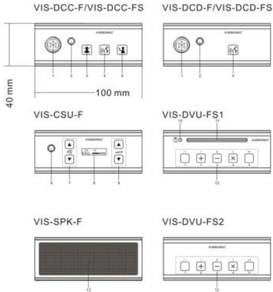
Figure 3.5.1.1 Front view of VIS-DCC/DCD/CSU/DVU/SPK-F/FS/FS1/FS2
