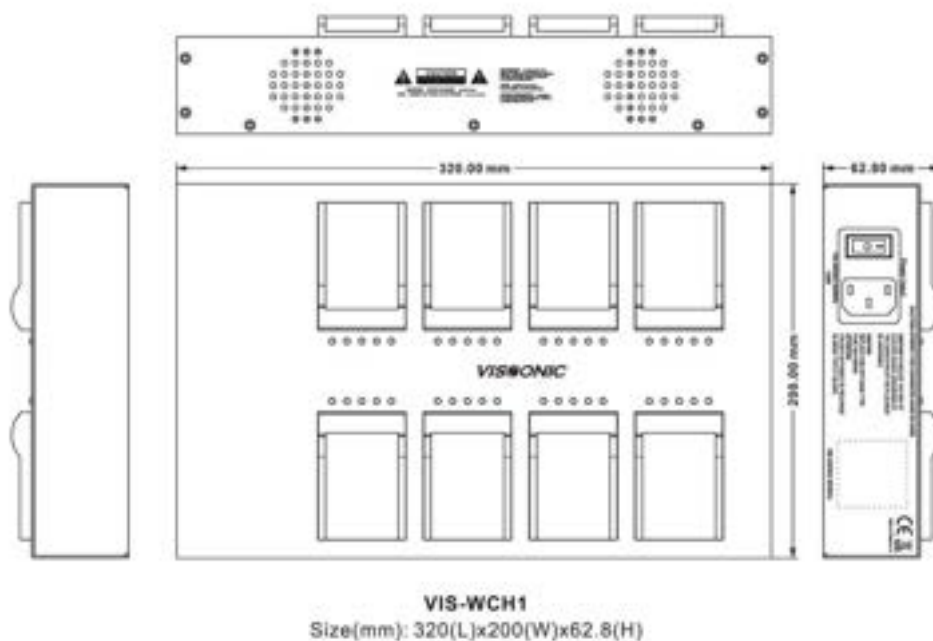
Figure 3.6.1.8 VIS-WCH1 charger for battery
