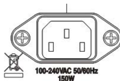
Figure 2.1.3.1 Power interface of the conference controller
