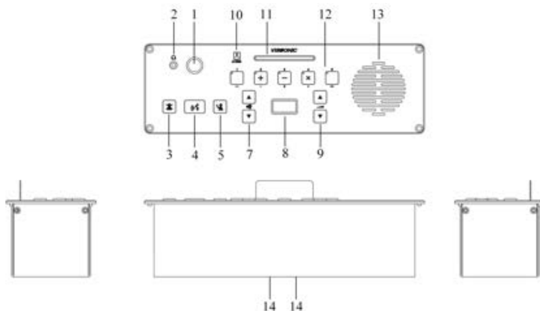
图 3.5.1.3 VIS-FFC/FFD-F1/F2 flush-mounting unit
