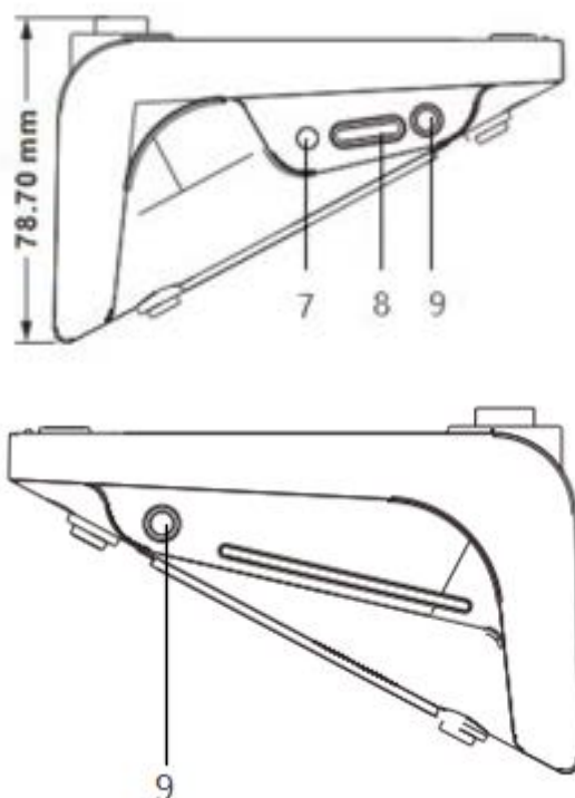
Figure 3.3.1.2 Left view and right view of VIS-MAU-T
