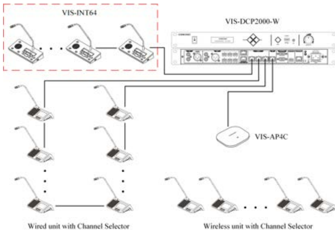
Figure 4.2.1 VIS-INT64 connected to controller
