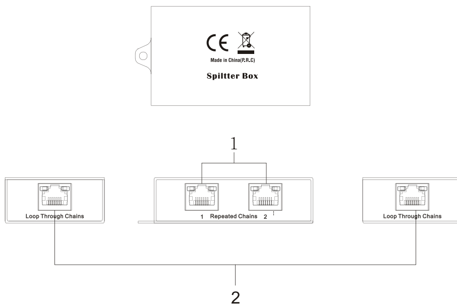
Figure 4.2 Front and rear panels of VIS-CNB and top cover
