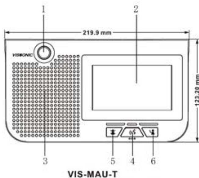
Figure 3.3.1.1 Top view of VIS-MAU-T
