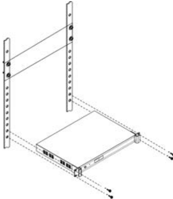
Figure 2.1.2 Mounting the conference controller
