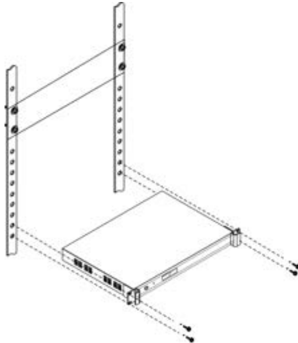
Figure 2.1.2 Mounting the conference controller
