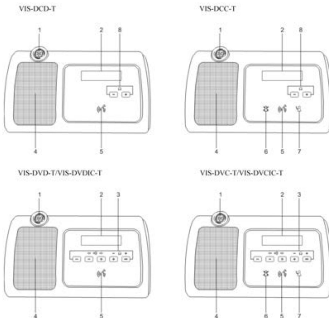
Figure 3.1.1.1 Top view of wired units VIS-DCC/DCC/DVC/DVD/DVCIC/DVDIC-T
