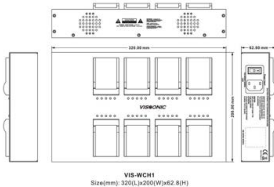
Figure 3.6.1.8 VIS-WCH1 charger for battery
