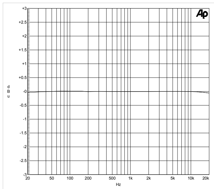
Z4MK4/Z8MK4 Music Output Frequency Response
