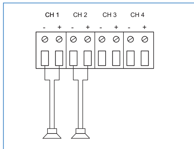
fig.6: Output Wiring
