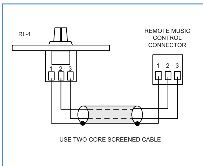
fig.5: RL-1 Wiring
