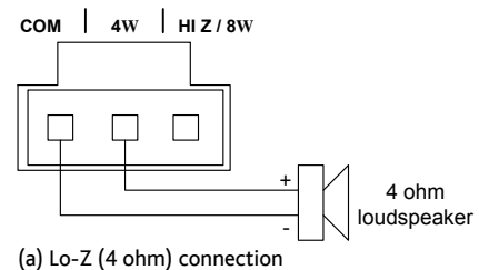
(a) Lo-Z (4 ohm) connection
