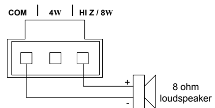
(b) Lo-Z (8 ohm) connection
