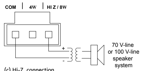
(c) Hi-Z connection
