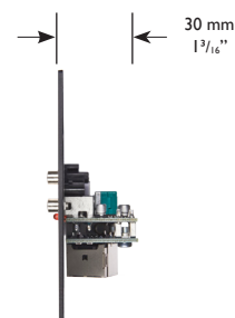
LE-1 side view
