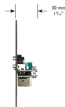
LE-1A side view
