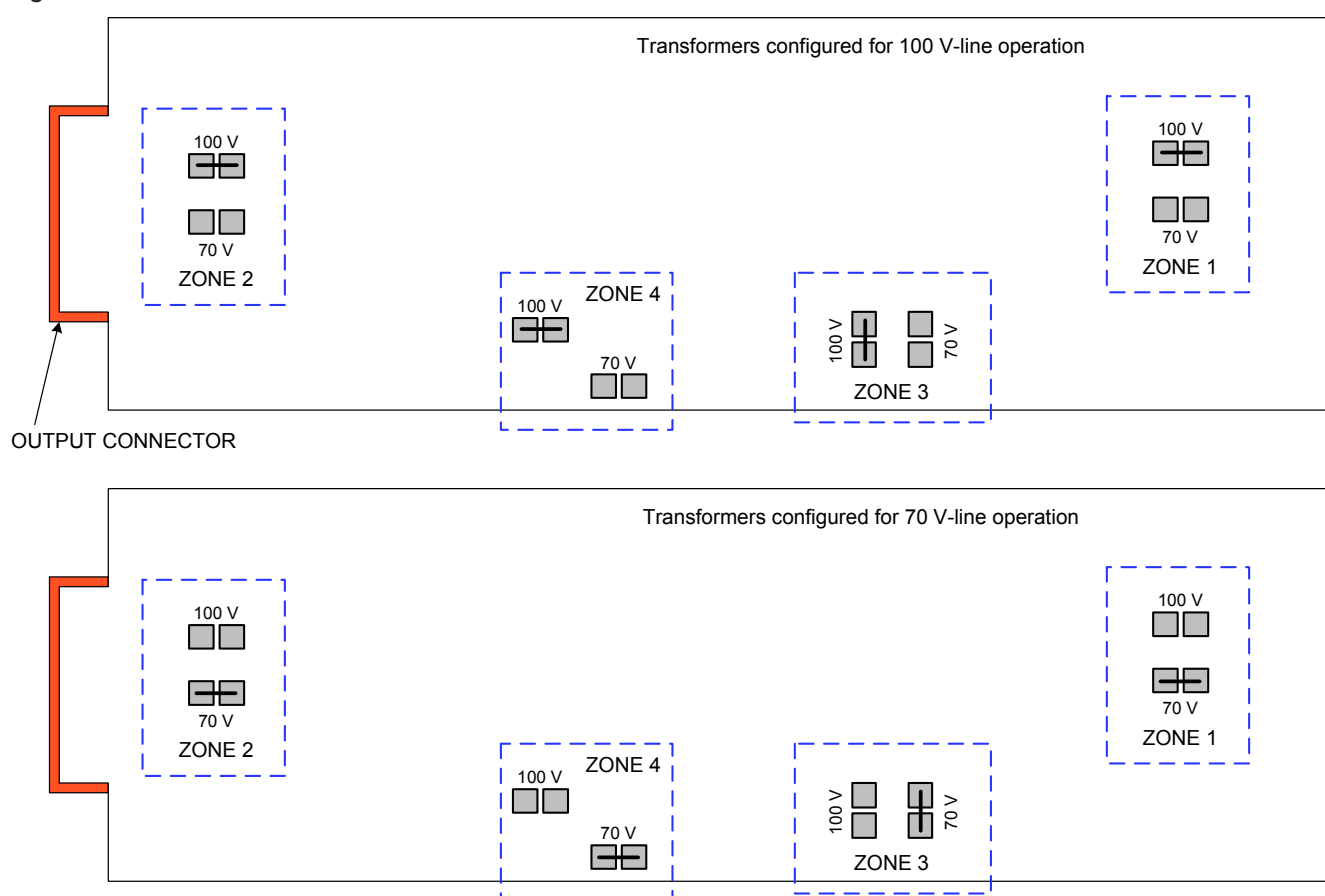
SOLDER SIDE OF PCB, SHOWING APPROX. LOCATIONS OF WIRE LINKS
