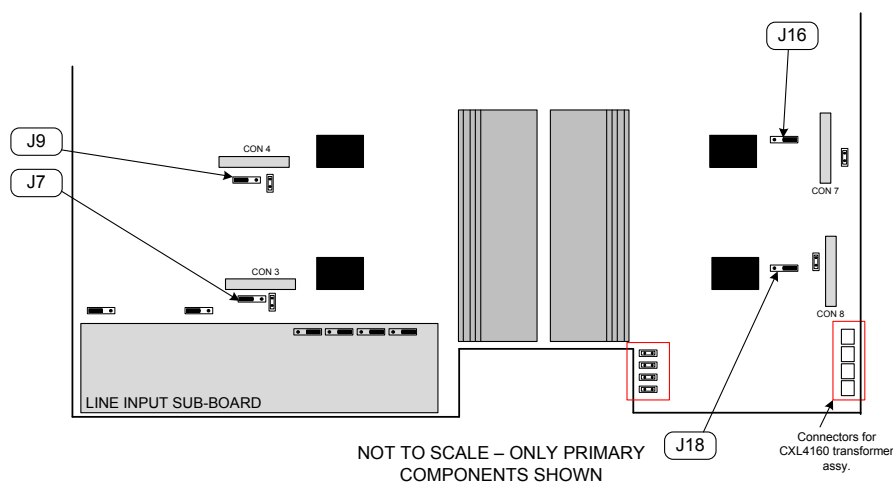
46-50 Jumper locations.
