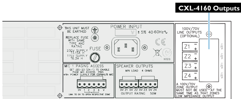
46-50 Rear Panel
