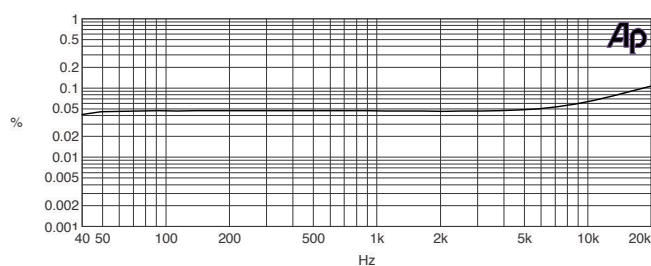
CXL400T & VTX4400 CH1 THD+N, 25 Ohms, 400W, BW 80kHz
