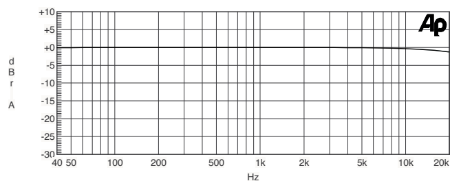
CXL200T & VTX4240 CH1 Frequency Response, 50 Ohms, 200W
