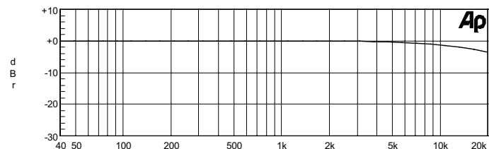
CXL100T, CX-A6 CH1, Frequency Response, 100 Ohms, 100W
