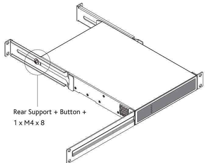
Diagram 4B CXARack Support hardware. 2 positions.
