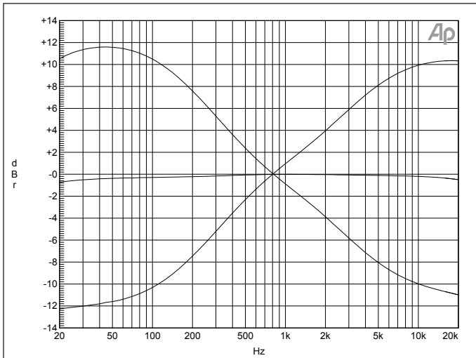
46-80 Line Input Tone Controls
