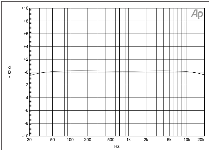
46-80 Line Input Frequency Response
