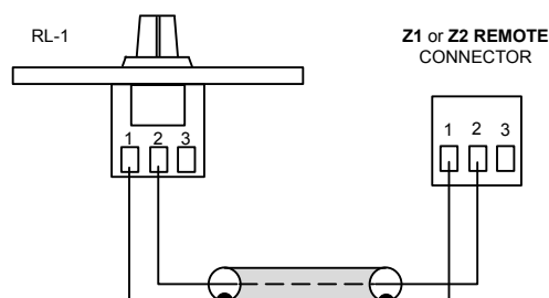
REMOTE LEVEL CONTROL WIRING
