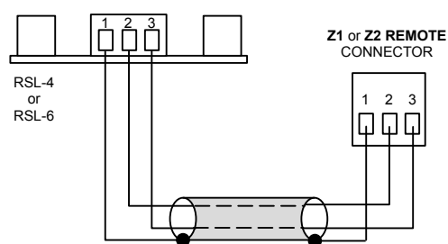
REMOTE SOURCE & LEVEL CONTROL WIRING
